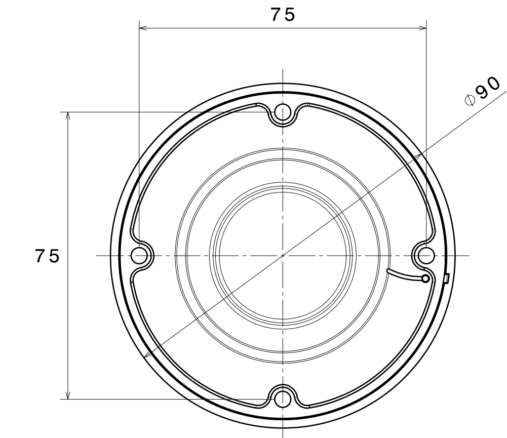
Bottom view
