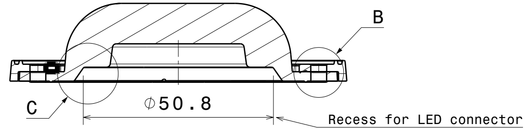
Section view A-A
